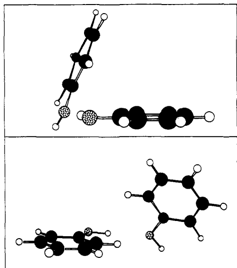
Figure 20. Two views of the most probable structure of the neutral phenol dimer. (Taken from ref 178.)
