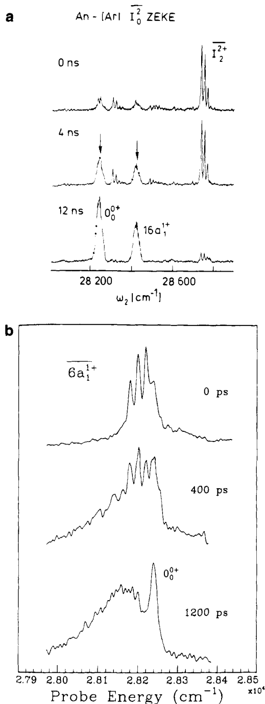
Figure 10. ZEKE spectra of aniline (An) complexes to monitor the dynamics in the S_1 state (dissociation and IVR). (a) ZEKE spectrum of An-Ar via the S_1 \bar{I}_0^2 level ( 762 \text{ cm}^{-1} , i.e. ca. 300 \text{ cm}^{-1} above the dissociation energy of the S_1 state) of the complex as a function of the delay time between pump and probe laser. The features indicated by arrows are product states of the aniline monomer which grow with increasing probe delay time. (Taken from ref 125.) (b) ZEKE spectrum of An- \text{CH}_4 via the S_1 6a_1^1 level of the complex as a function of the delay time between pump and probe laser. The broad structure in the lower trace is due to IVR to the intermolecular van der Waals modes. The sharper peak at late time is the vibrationless aniline dissociation product. (Taken from ref 126.)
