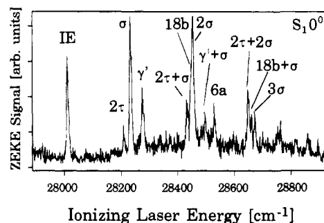
Figure 15. ZEKE spectrum of the 3-fold deuterated 1:1 phenol–water complex, [\text{Ph}-\text{H}_2\text{O}]\text{-d}_3 ( i.e. PhOD– \text{D}_2\text{O} ), via the S_1 0^0 level. (Taken from ref 135.)
