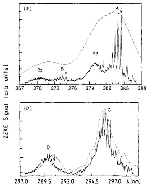
Figure 5. Threshold photodetachment (ZEKE) spectrum of I^-CO_2 (solid lines) and conventional photodetachment spectrum (dotted lines). The arrows indicate the band origins. See text for details. (Taken from ref 74.)
