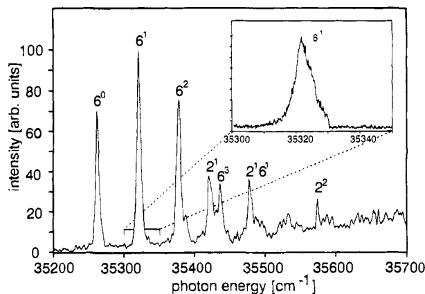
Figure 4. Nonresonant one-color, two-photon ZEKE spectrum of the NO dimer. The inset shows a high accuracy scan of the rotationally broadened 6^1 band. (Taken from ref 51.)
