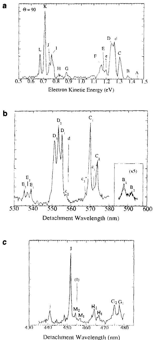
Figure 6. (a) Photodetachment spectrum of Si 2 - with laser polarization perpendicular to the direction of electron detection (the detachment wavelength is 355 nm) (taken from ref 97); (b) ZEKE spectrum of Si 2 - showing transitions to the triplet states of Si 2 (taken from ref 97); (c) ZEKE spectrum of Si 2 - showing transitions to the singlet states of Si 2 (taken from ref 97).
